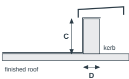
KERB SECTION
